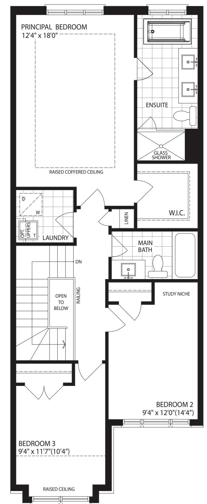
SECOND FLOOR ELEV. C
